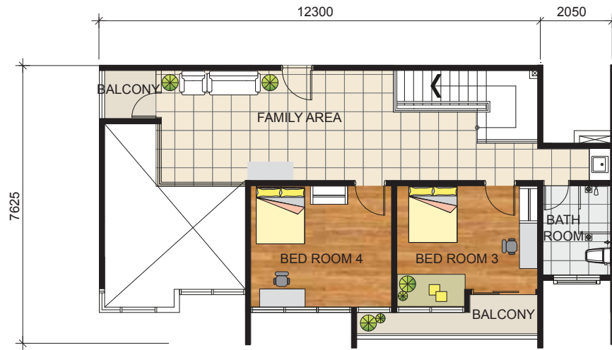
DUPLEX PENTHOUSE (UPPER FLOOR)-TYPE H
